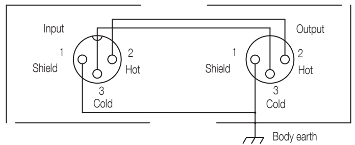
Circuit diagram
