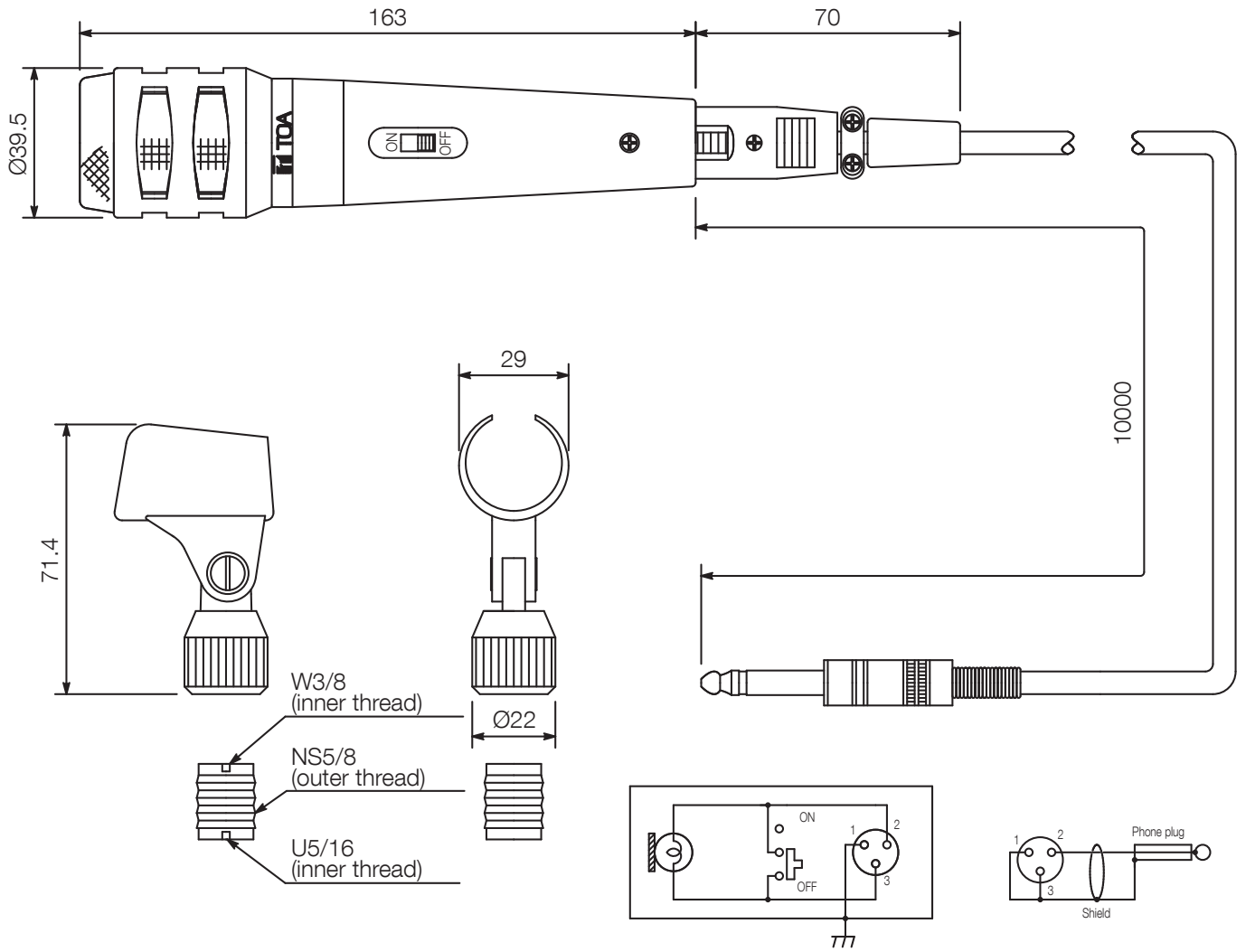
Circuit Diagram
